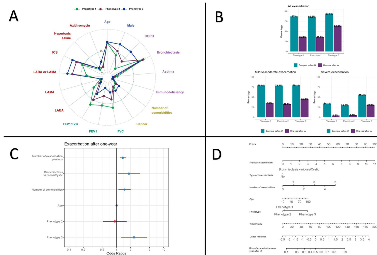
Fig. 1. Panel A: Distribution of clustered characteristics by phenotype; Panel B: Exacerbation one-year pre-post IA according to phenotypes; Panels C and D: Multivariate model for risk of exacerbation one-year after IA. (A) Radar plot showing the prevalence or standardized mean (0–1) of clustered characteristics for clinical phenotype identification. Clustering was performed using k-prototypes with multiple imputation on sociodemographic information (blue), underlying respiratory diseases (purple), comorbidities (yellow), pulmonary function (green) and pharmacological treatments (red). Abbreviations: COPD, chronic obstructive pulmonary disease; FVC, forced vital capacity; FEV 1 , forced expiratory volume in 1 second; ICS, inhaled corticosteroids; LABA, long-acting beta2 agonist; LAMA, long-acting muscarinic antagonist. (C) Forest plot with Odds Ratios and confidence interval for predictors of exacerbation model. (D) Nomogram to predict risk of exacerbation after one-year IA.
