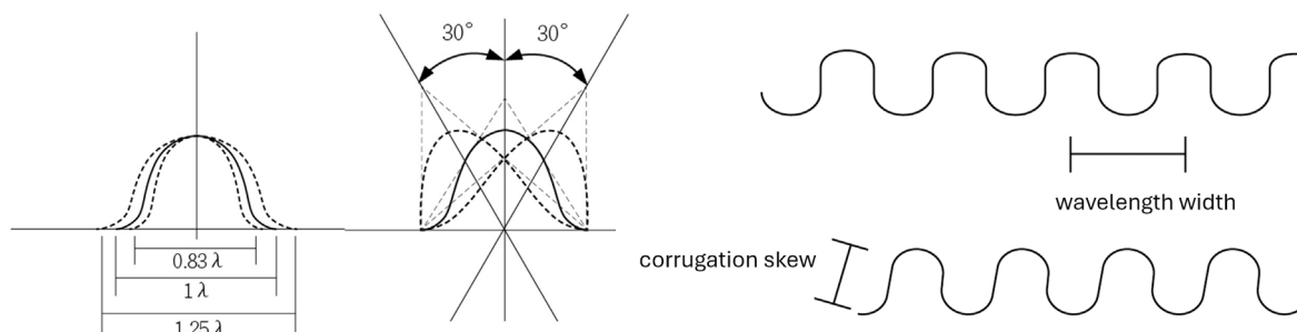
Fig. 1. 3wavelength width and 3corrugation skew.
